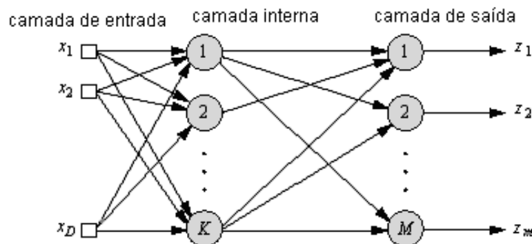
Figura 3-3 – Topologia do Perceptron MLP
